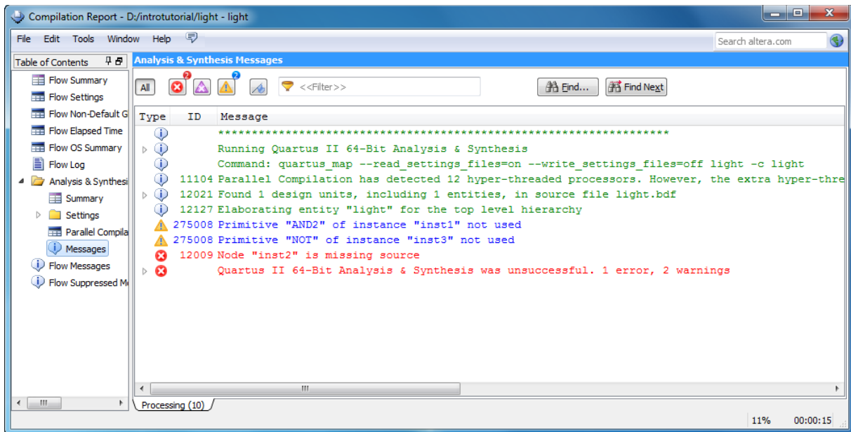
Figure 23. Error messages.
