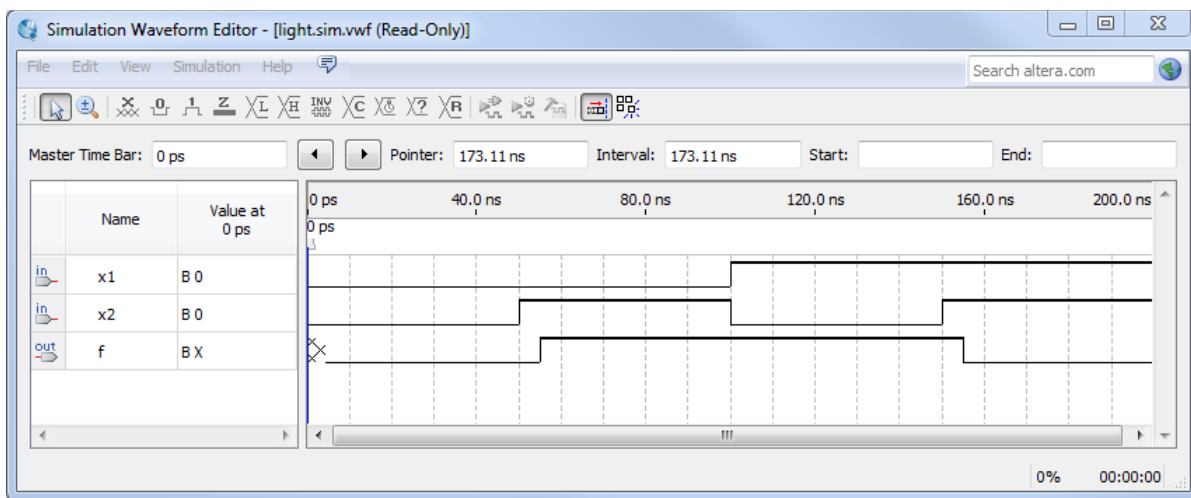
Figure 38. The result of timing simulation.
